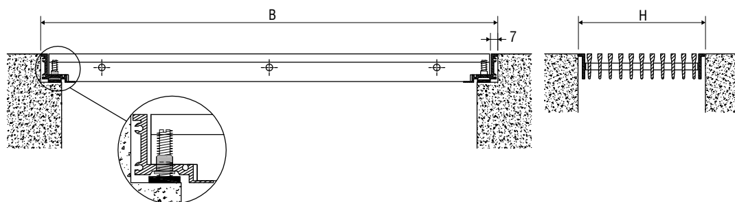
BPAR+CBPAR
